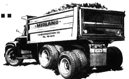
Factory-built tandem-axle T-800. 42,000 lbs. GVW, 65,000 lbs. GCW. Two V-8's (200 or 212 h.p.).
