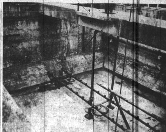
THE ABOVE PICTURE was taken Wednesday evening when all eight aeration tanks were emptied to enable contractors to install the air pipes shown along the bottom of the tank. Each tank holds 66,000 gallons of water at a depth of 10 1/2 feet. City officials believe that the addition of the new equipment will answer, in part, a citation placed on the city by the state's Water Resources Commission for pollution of the Rouge river.
