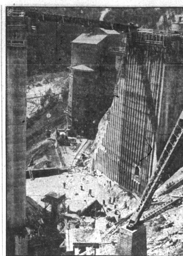
HIGH-SIDED HOLE —Only space left to fill in 564-foot-high Hungry Horse Dam, way up in western Montana, is block number 25 shown above. Two concrete pours will complete placement of all concrete used in the dam. Seen beyond the dam is the 139-foot-high concrete mixing plant. It turned out more than three million yards of cement for the dam, its power plant and other buildings used in construction of the dam which was built under direction of the Bureau of Reclamation, Department of the Interior. President Truman turned on the power Oct. 1 and dedicated the project which was completed 14 months ahead of schedule by the General Shea-Morrison Co. at a cost of $103,000,000.
