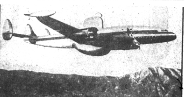
BUBBLE BELLY —Flying out of Burbank, Calif., a Super Constellation laboratory ship, with a shark-like fin on top of its fuselage and a bulbous protrusion beneath, bears aloft the Navy's new WV-2 radar equipment. The electronic device is designed to act as a flying sentinel in this country's civil defense plans.
