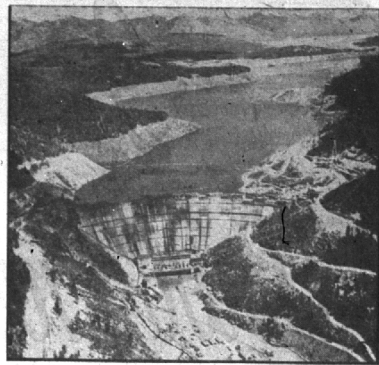
HUNGRY HORSE READY TO FEED —In the shadows of white-capped mountains, construction crews work at top speed to complete construction of Hungry Horse Dam on Montana's Flathead River by autumn. The Bureau of Reclamation project will raise to a height of 364 feet, store 3,500,000 acre feet of water, and add 300,000 kilowatts of power to the northwest power pool.
