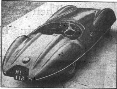
"FLYING DISK" —This may look like a "life boat" from a flying saucer, but in reality it's only a new auto being tested by Alfa Romeo in Milan, Italy. Built along entirely new principles, the "Flying Disk" is powered by a six-cylinder engine with three double-body carburetors, and can develop about 200 horse power, with a maximum speed of 120 m.p.h.
