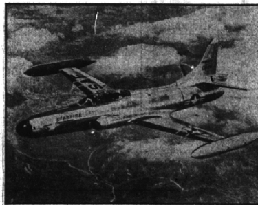
“SHE'S A HONEY”—Designed to guard our shores against enemy bombers, this new Lockheed P-94-C Starfire, jet-fighter interceptor climbs to 45,000 feet in a twinkling and zooms along in all weather “in the 600-mph class.” Its “bubble nose” houses instruments that electronically track down enemy aircraft. The “almost automatic” Starfire is the first fighter plane to have all-rocket armament, carrying 24 rockets, 2.75 in. size. Said test pilot Tony Lovice after landing at Palmdale, Calif., “She's a honey.”
