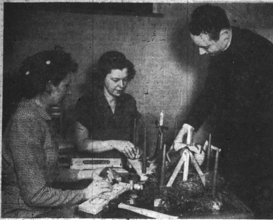
MRS. CARL AARON MRS. RAYMOND SIMANCEK REV. PAUL SHIPPERT Preparing Advent wreaths at Ascension Lutheran church
