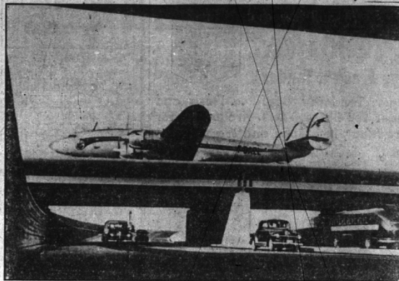
An Air France Constellation taxis over the world's first roadway underpass built to permit the simultaneous movement of aircraft and surface vehicles at New York's International Airport. The underpass, considered a major engineering feat, drops to below sea level at the point pictured above. The roadway, retaining walls and overpass comprise a 92,000-ton "concrete boat" built to withstand pressures from below sea level.
