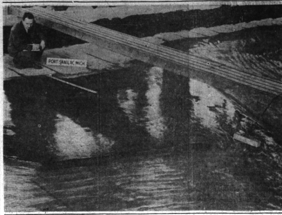
UNIVERSITY OF MICHIGAN research will assist engineers in building harbors of refuge for small craft at Port Sanilac and Port Austin, two Michigan towns on Lake Huron. Pictured above is the "Port Sanilac" harbor inside the University's wave-tank laboratory as tests are run to determine the proper location and length for a breakwater. Waves, which out in Lake Huron would be seven feet high, are rolling in as Ernest F. Bealer, associate professor of civil engineering, notes the results.
