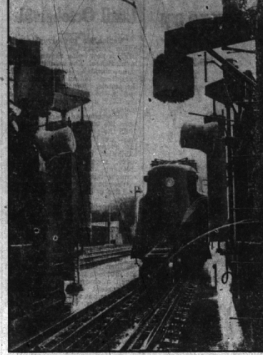
Now they're sending locomotives to the laundry. This is a new semi-automatic locomotive washer at Pennay's New York yard, where the 2 hours, 55 minutes required for hand washing has been cut to 13 minutes by a set of revolving pinwheel sprays of hot water and steam, and horizontal and vertical brushes. Four men operate the 300-foot installation, which will launder 100 engines in 24 hours.
