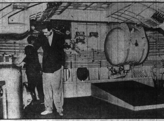
Idea of the size of Howard Hughes' huge $20,000,000 flying boat, world's biggest plane, is given by this interior view showing Hughes inspecting equipment. The plane is nearing completion at Terminal Island, Calif.
