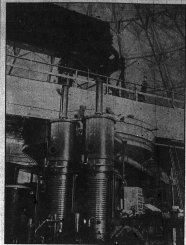
Tiny figure of man, upper right, gives you an idea of size of University of California's 184-inch cyclotron in this first photo of the atom smasher. Work on the machine was interrupted during the war, but it will be ready for operation this fall. Manhattan District—Army's atom bomb outfit—is assisting in the university's atomic research.
