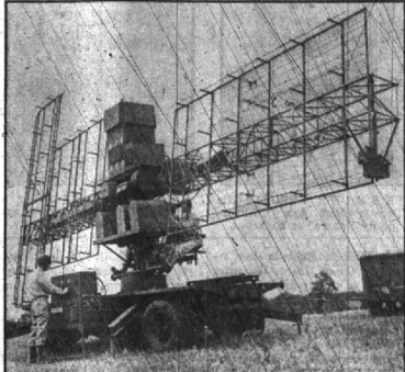
This is a mobile radar unit. Man at left is operating the keyer and modulator. Three men on seats behind triple-antennae are operating vertical position scope (short for oscilloscope), horizontal position scope, and range scope. These three cathode ray oscilloscopes plot the echo resulting when the beams meet a plane or other solid mass.
