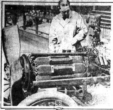
Ever since the close of the World war G. E. Franklin has been working on a new type of airplane motor which he plans to manufacture in Kansas City, Mo., in the near future. It weighs 359 pounds and develops 400 horse power. It features 16 air cooled and valveless cylinders and its inventor declares it will revolutionize the motor car and airplane industries. The motor is shown above with Franklin beside it.
