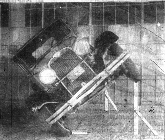
At this 42-degree angle, the Dodge Brothers Victory Six is trying to right itself and get back on "all fours." Engineering experiments have proved that the car can be tilted 46 1/2 degrees. The low center of gravity and the unique battleship type of body construction in the Victory Six are regarded as important safety features.
