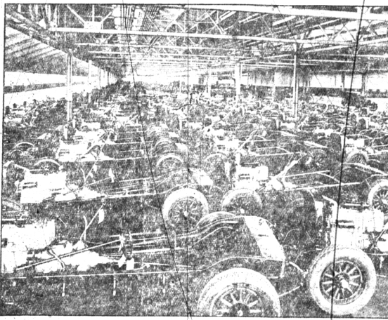
The above picture shows the interior of Dodge Brothers' mammoth new plant in which the company's line of fine six-cylinder motor cars is being built. Hundreds of six-cylinder chassis are shown covering every available inch of floor space in the half-mile-long building. Production of the new line was started early in May with an initial daily output of about 50 cars. This rate has been stepped up from week to week and the plant is now turning out about 150 cars a day. Shipments to dealers were started the middle of May and have been made in such volume that practically all dealers have been supplied. Production will be still further increased in June and by the middle of the month daily output will be approximately 300 per day.
