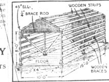
Garage Frame Made With Pipe and Fittings.
