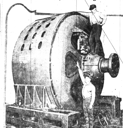
This is one of the four electric motors supplying 1,000 horse power to one of the propellers on the U. S. S. Maryland. The mammoth motor is twelve feet high and weighs 22 tons.
