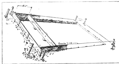
Forms for a Concrete Feeding Floor.
